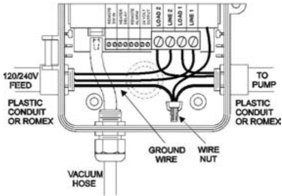
Fig. 4.A Wiring with Non-Metallic Conduit
