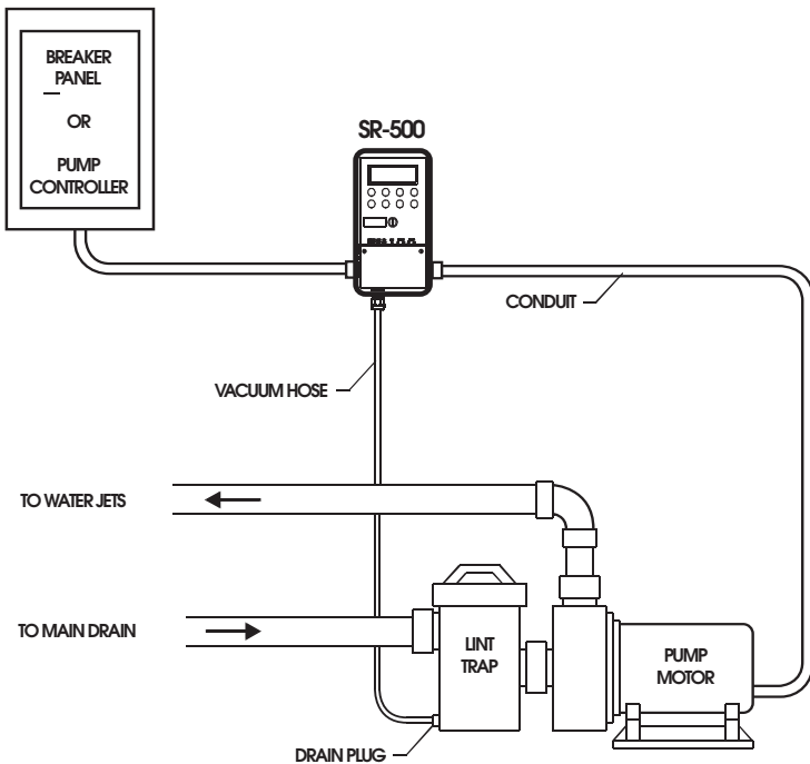
Fig.1: System Diagram
